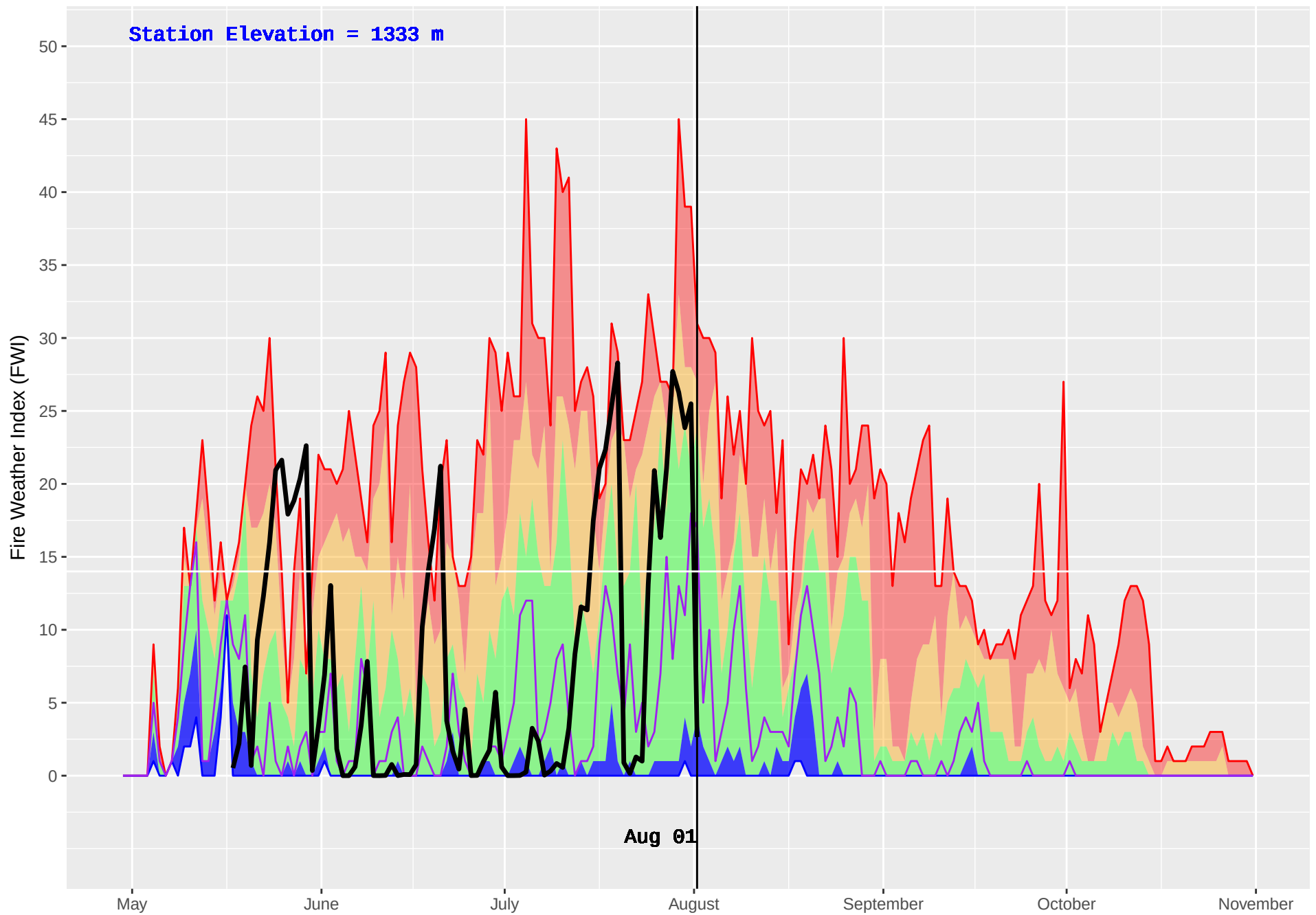
GOLDSTREAM 2 (919) : Historical (2005–2016) and Current (2018) Daily Fire Weather Index (FWI)
