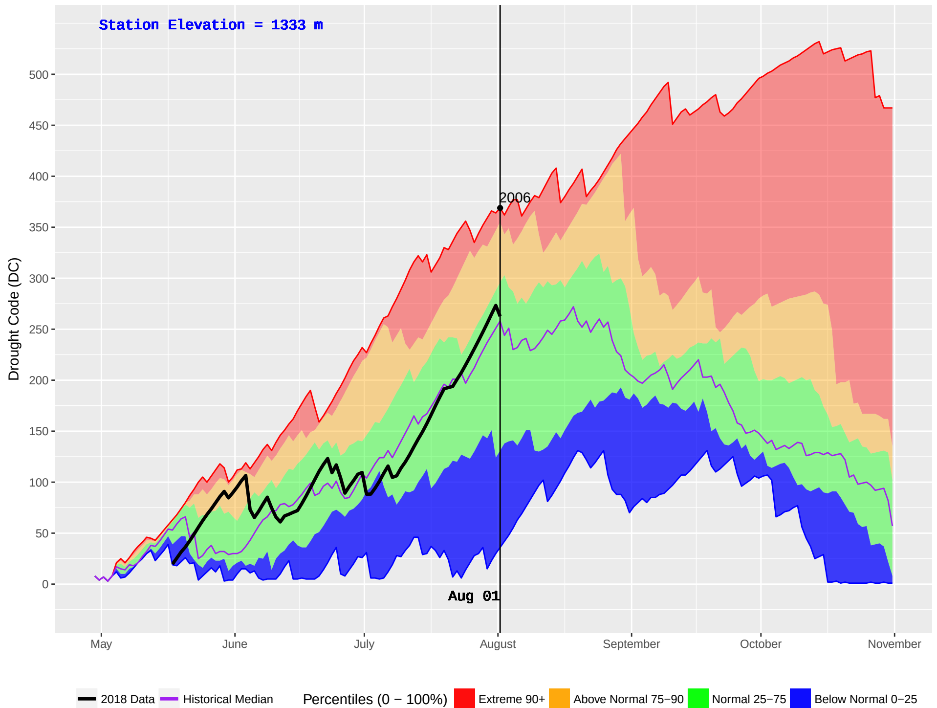
GOLDSTREAM 2 (919) : Historical (2005–2016) and Current (2018) Daily Drought Code (DC)
