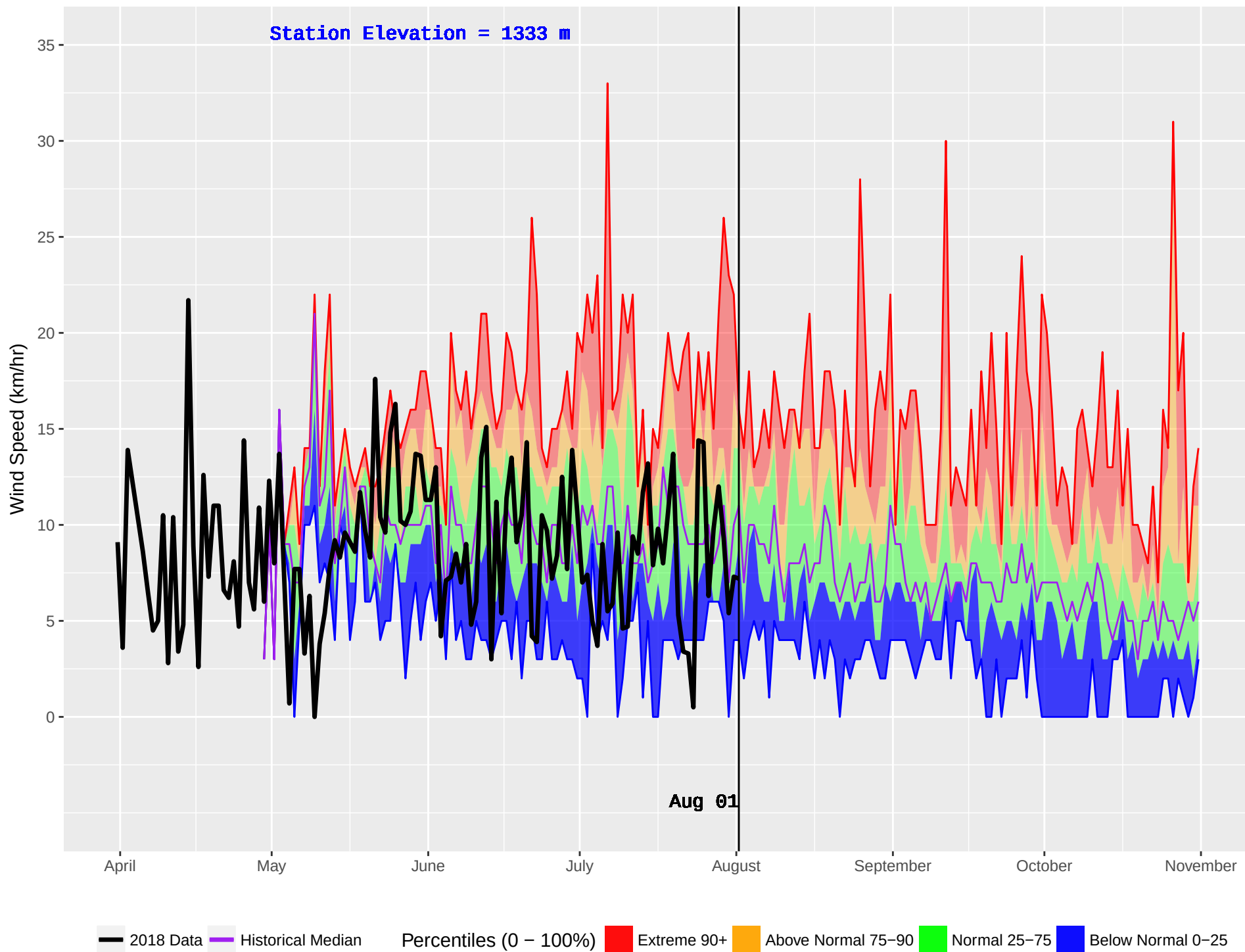
GOLDSTREAM 2 (919) : Historical (2005–2016) and Current (2018) Daily Wind Speed
