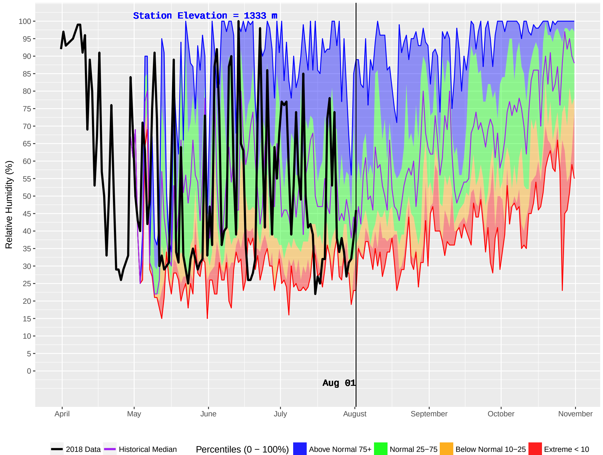
GOLDSTREAM 2 (919) : Historical (2005–2016) and Current (2018) Daily Relative Humidity
