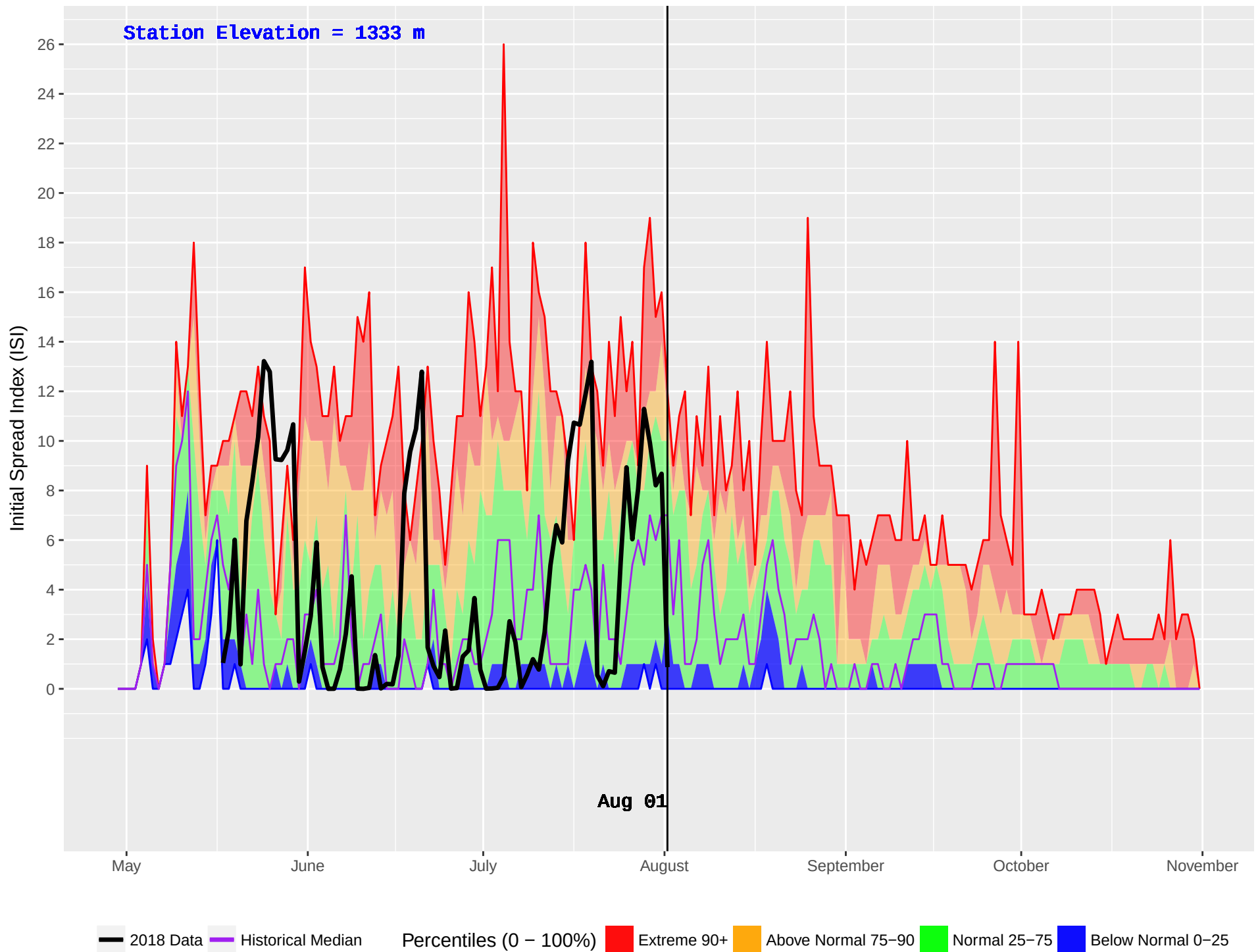
GOLDSTREAM 2 (919) : Historical (2005–2016) and Current (2018) Daily Initial Spread Index (ISI)
