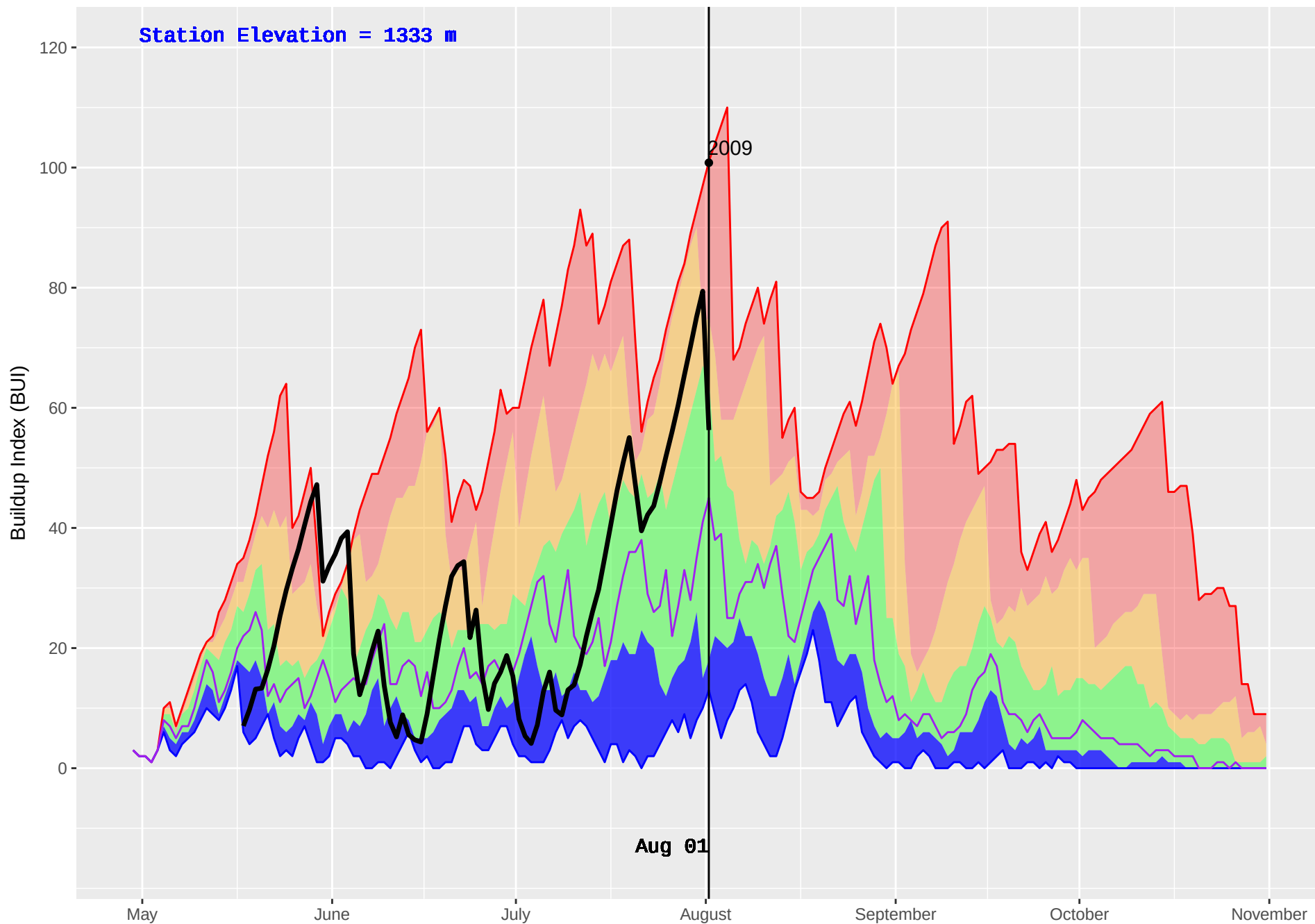
GOLDSTREAM 2 (919) : Historical (2005–2016) and Current (2018) Daily Buildup Index (BUI)
